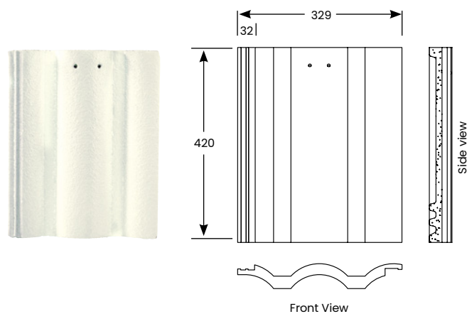
Concrete Elabana In Salt Spray
