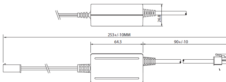
Speed Controller
