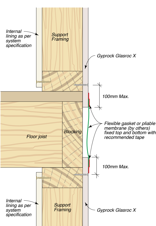
Figure 48: Intermediate Junction – Option 1
