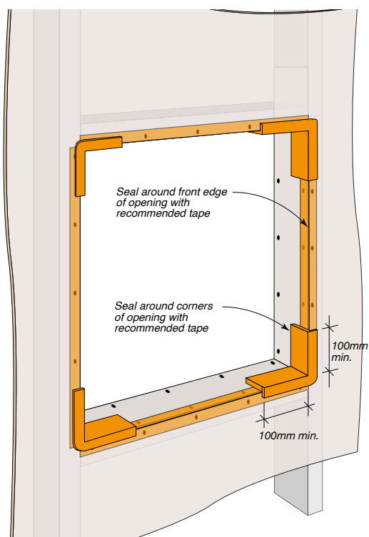
Figure 43: Treatment at Opening Step 2
