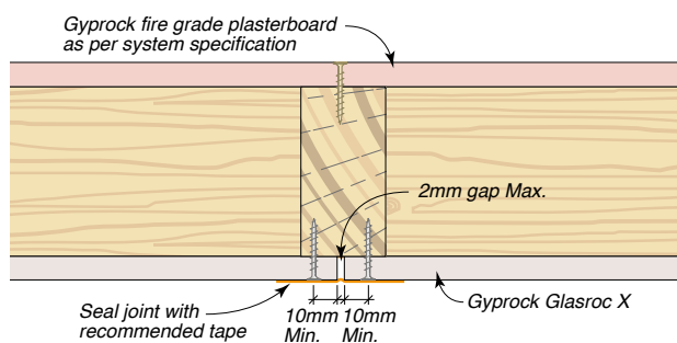
Figure 64: Vertical Junction – Tape
