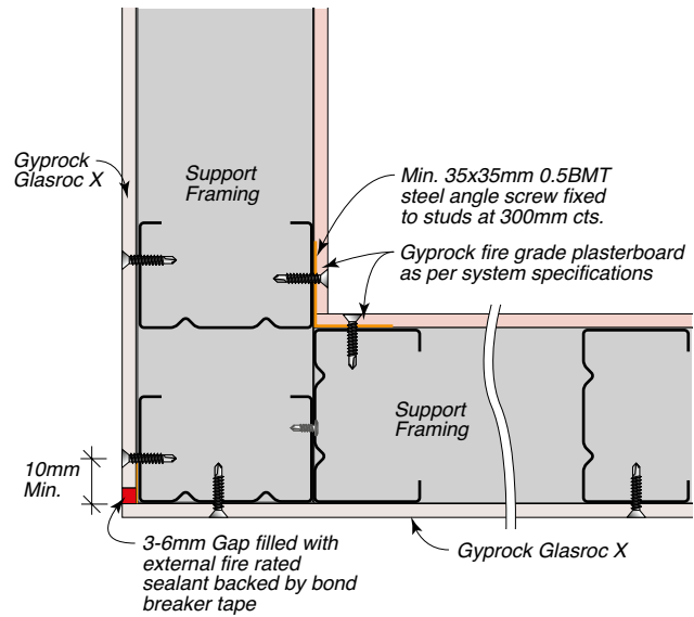
Figure 40: External Corner – Sealant
