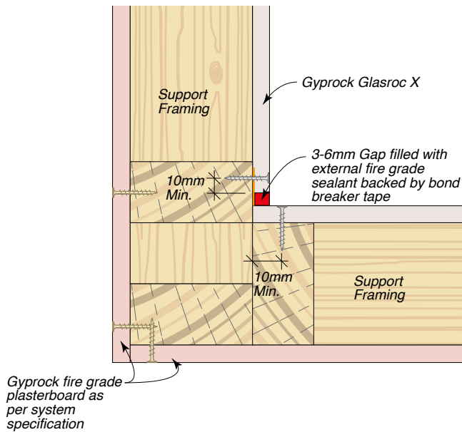
Figure 72: Internal Corner – Sealant
