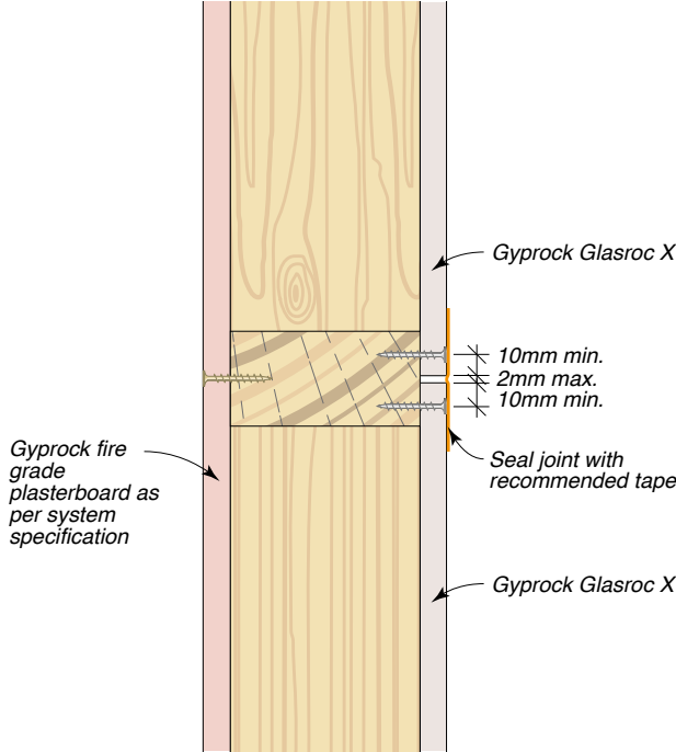
Figure 69: Horizontal Joint – Tape
