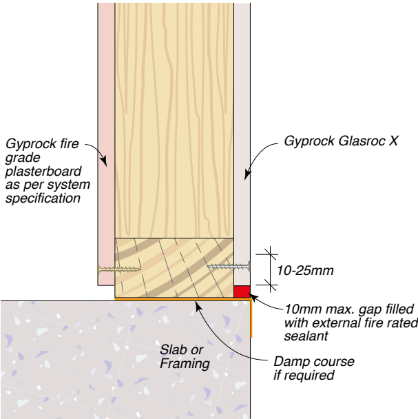
Figure 68: Base Detail – Sealant
