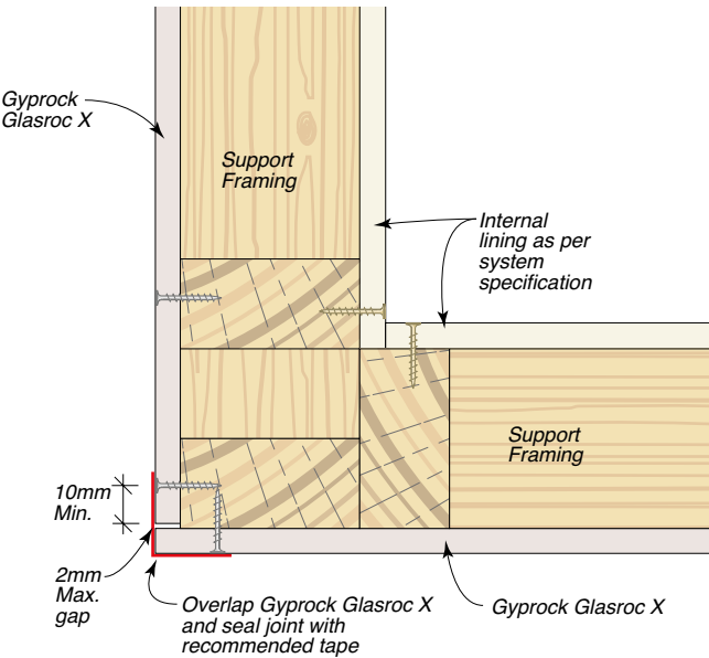
Figure 59: External Corner – Tape
