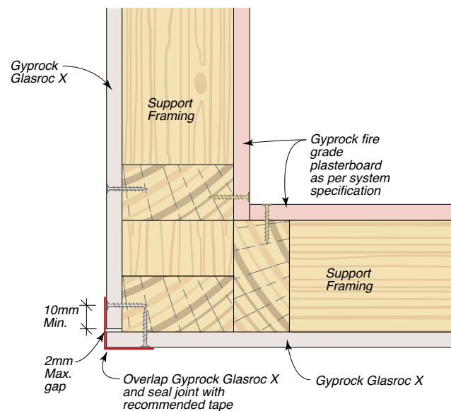
Figure 73: External Corner – Tape
