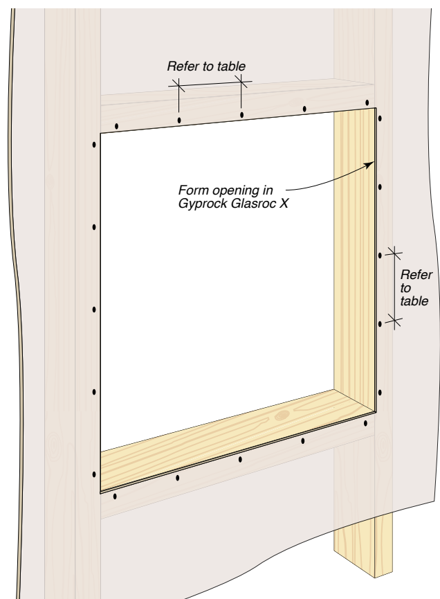
Figure 76: Treatment at opening Step 1
