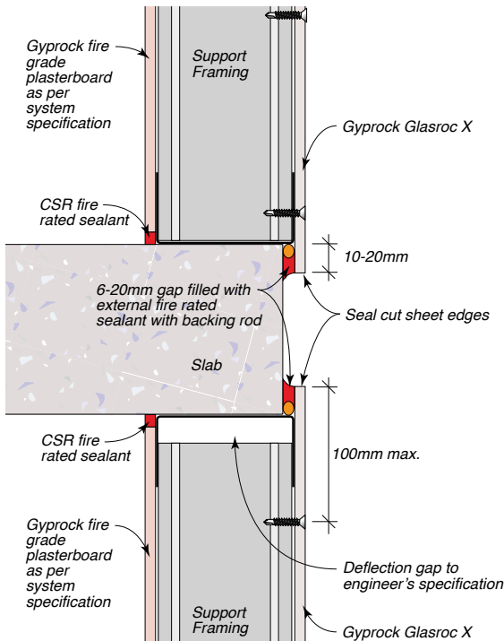
Figure 30: Intermediate Junction – Sealant
