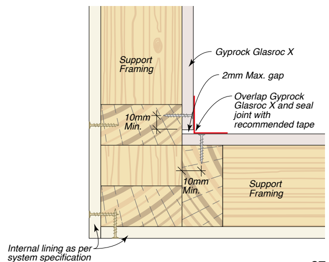
Figure 57: Internal Corner
