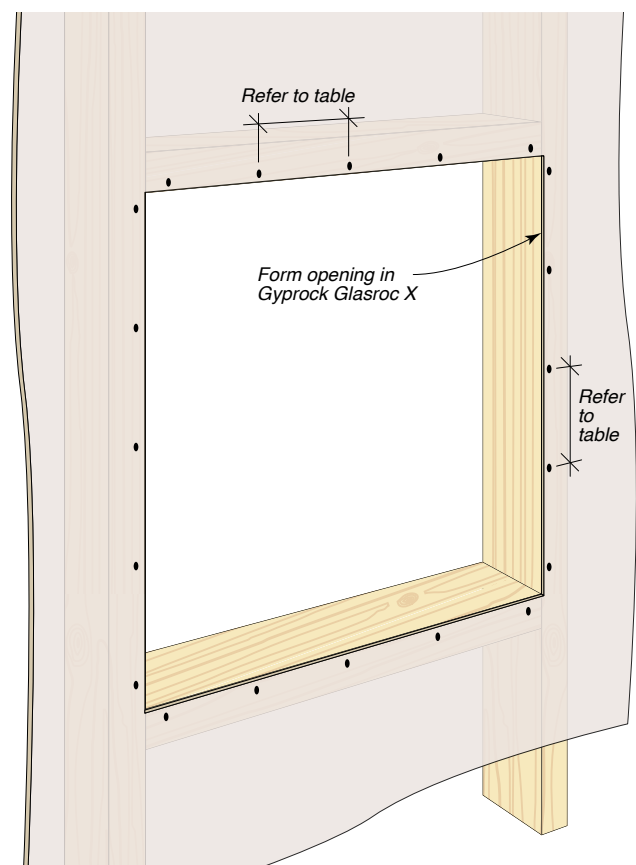
Figure 62: Treatment at Opening Step 1
