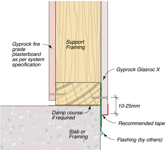
Figure 67: Base Detail – Tape
