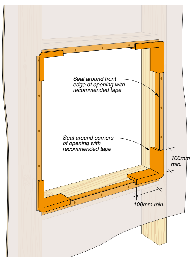
Figure 63: Treatment at Opening Step 2
