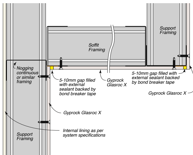
Figure 26: Soffit Junction – Sealant
