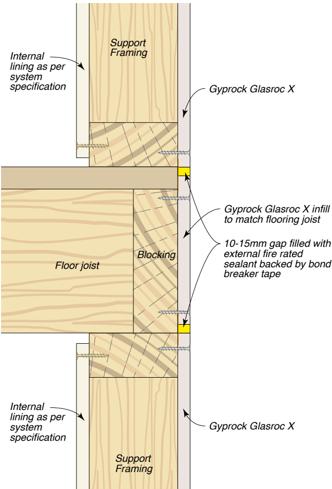
Figure 49: Intermediate Junction – Option 2
