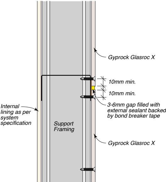
Figure 18: Horizontal Joint – Sealant
