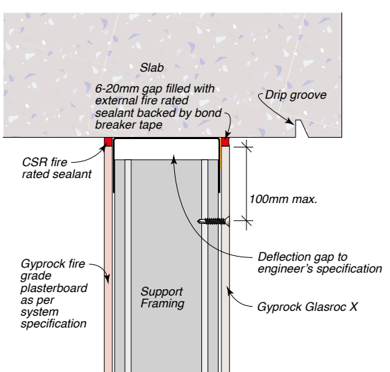
Figure 32: Head Detail – Sealant Option 2
