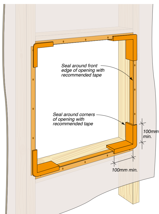
Figure 77: Treatment at opening Step 2
