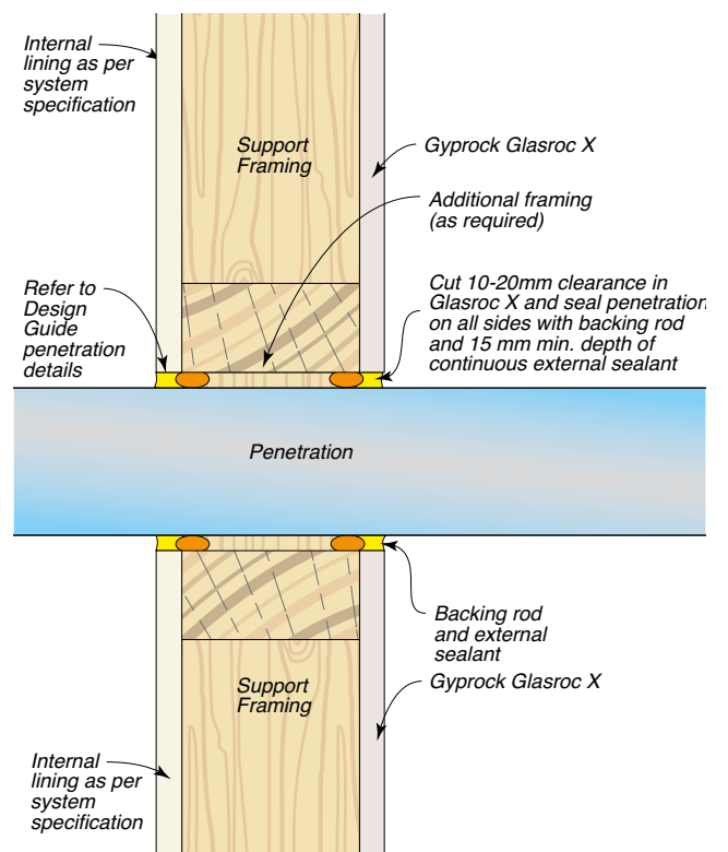
Figure 55: Junction at penetration – Sealant
