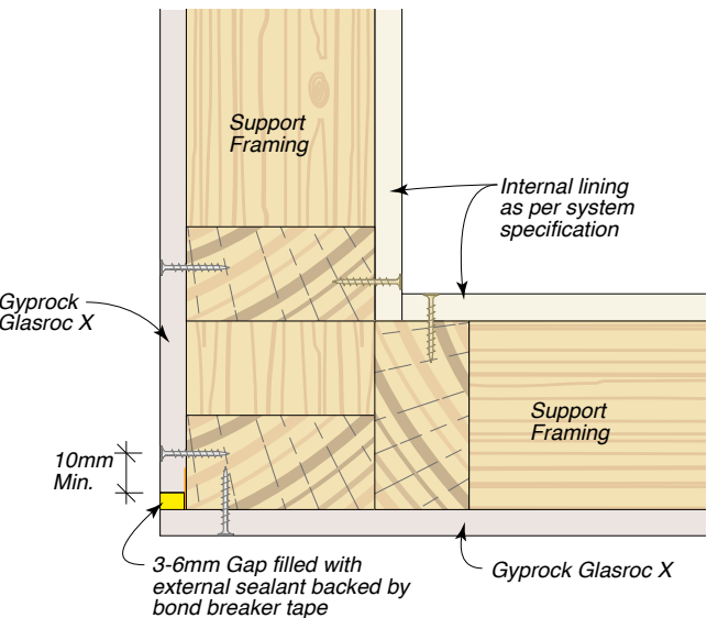
Figure 60: External Corner – Sealant
