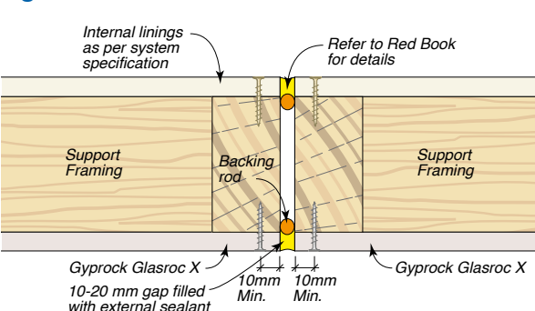
Figure 47: Vertical Control Joint – Sealant
