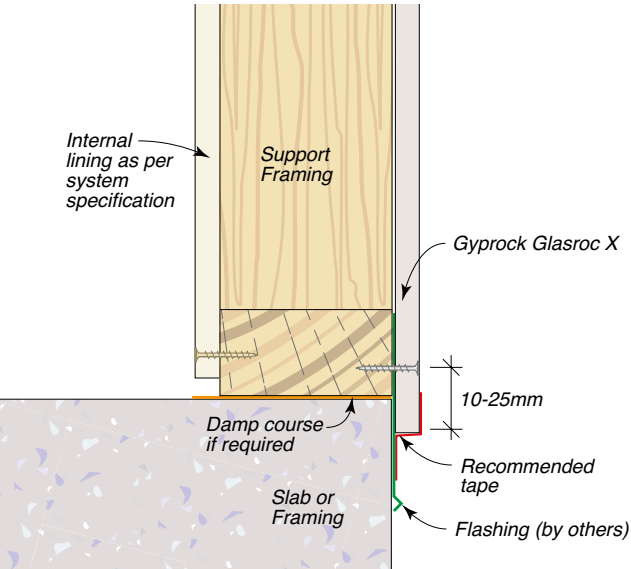
Figure 51: Base Detail – Tape Option 2
