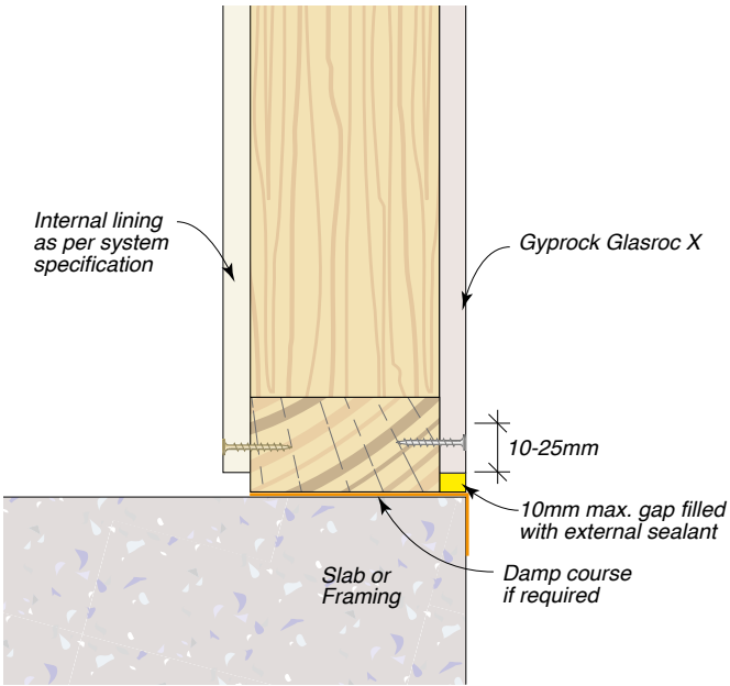
Figure 52: Base Detail – Sealant
