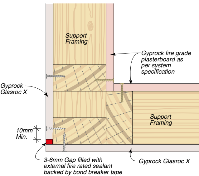
Figure 74: External Corner – Sealant
