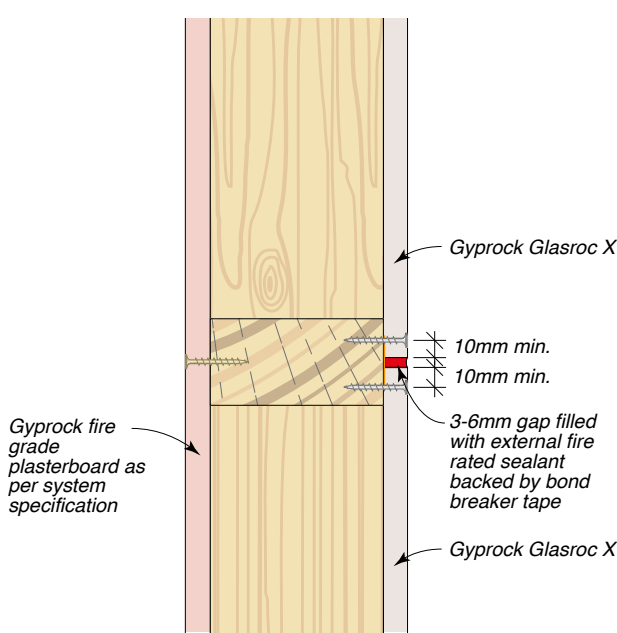
Figure 70: Horizontal Joint – Sealant
