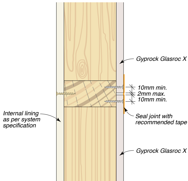
Figure 53: Horizontal Joint – Tape
