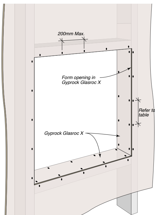
Figure 42: Treatment at Opening Step 1
