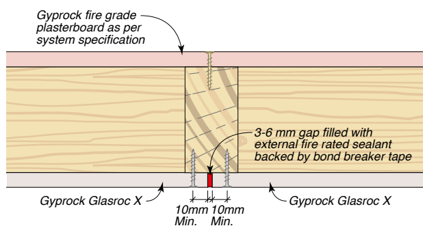
Figure 65: Vertical Junction – Sealant
