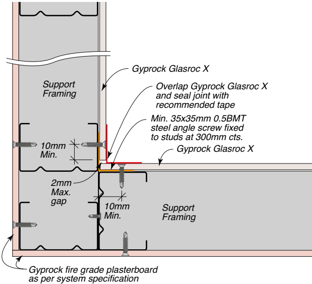
Figure 37: Internal Corner – Tape
