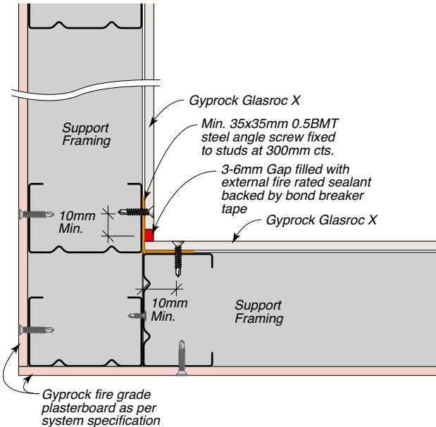
Figure 38: Internal Corner – Sealant
