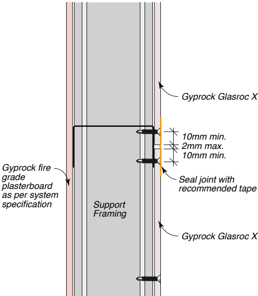
Figure 35: Horizontal Joint – Tape
