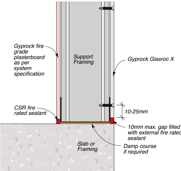
Figure 34: Base Detail – Sealant
