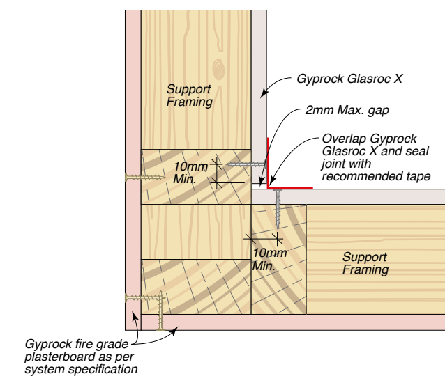
Figure 72: Internal Corner – Sealant
