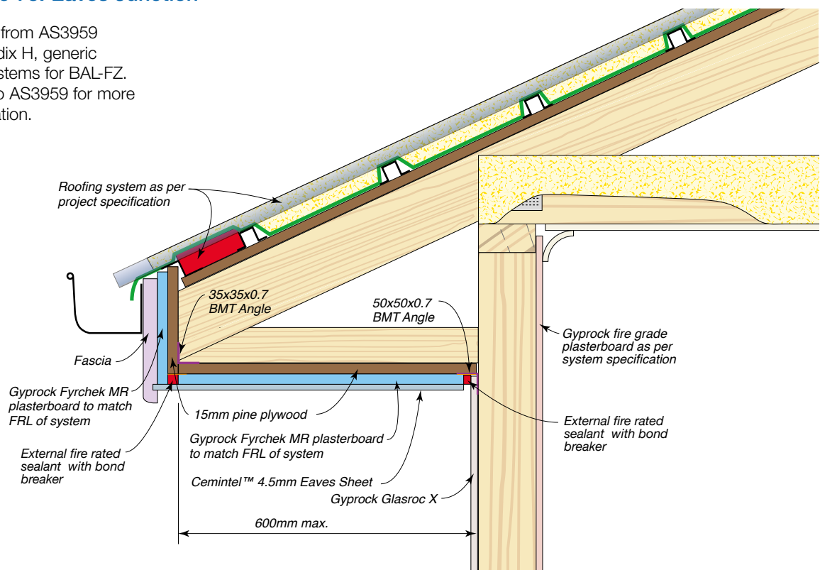
Figure 78: Eaves Junction
