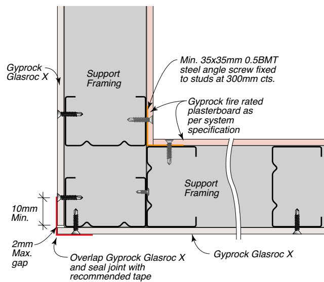
Figure 39: External Corner – Tape
