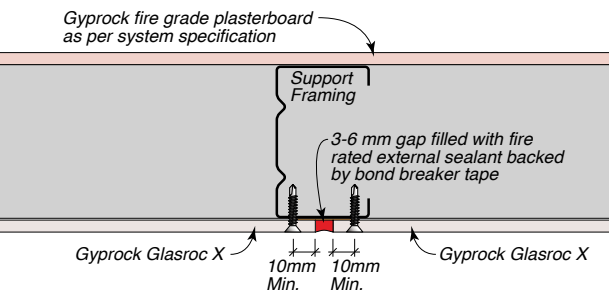
Figure 29: Vertical Junction – Sealant
