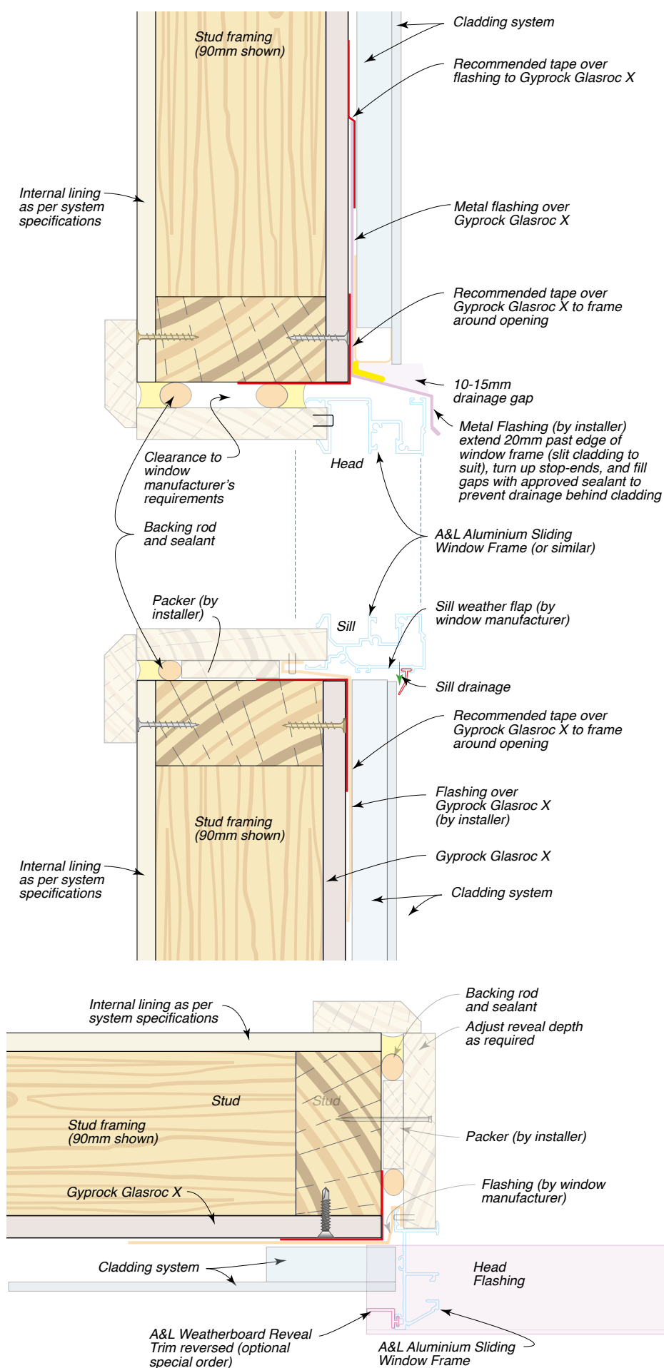
Figure 61: Window Penetration
