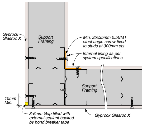
Figure 24: External Corner – Sealant
