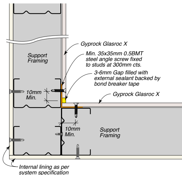
Figure 22: Internal Corner – Sealant
