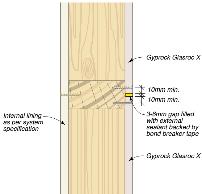
Figure 54: Horizontal Joint – Sealant
