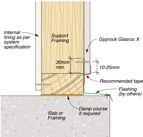
Figure 50: Base Detail – Tape Option 1
