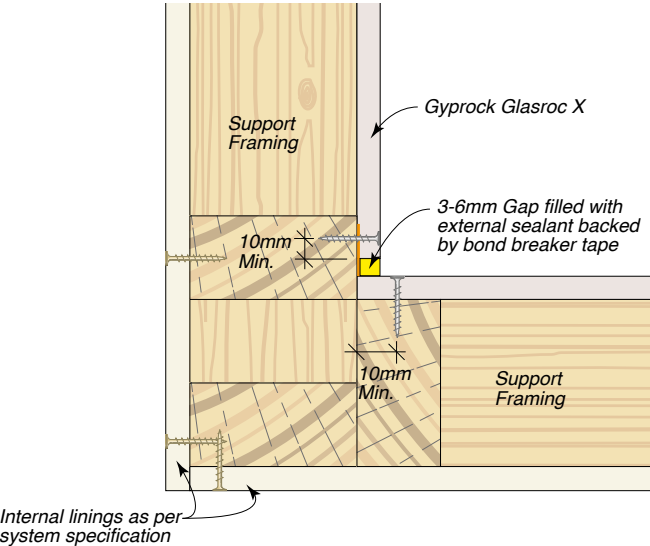
Figure 58: Internal Corner – Sealant
