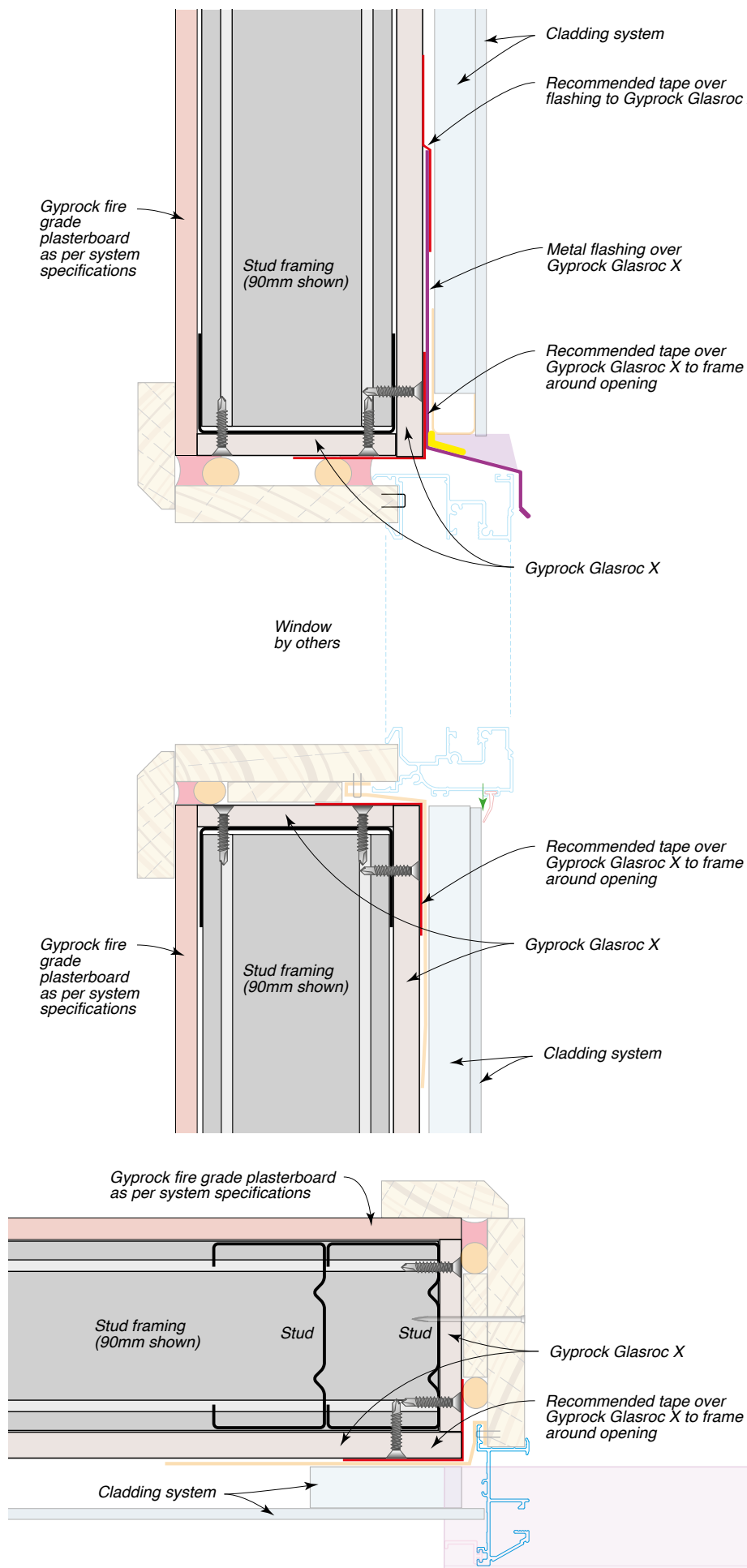
Figure 41: Window Penetration
