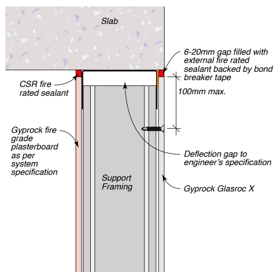
Figure 31: Head Detail – Sealant Option 1
