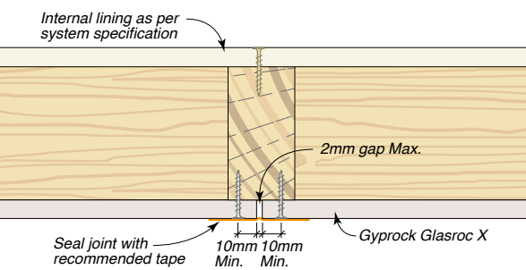
Figure 44: Vertical Junction – Tape
