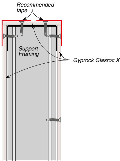
Figure 20: Parapet – Tape
