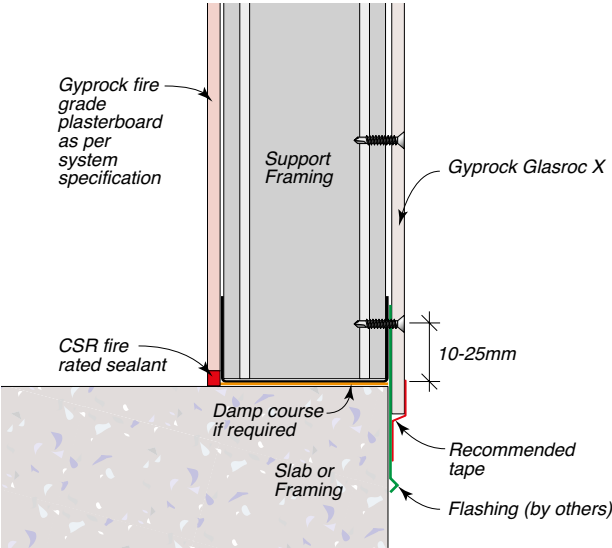
Figure 34: Base Detail – Sealant
