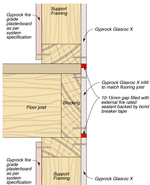
Figure 66: Intermediate Junction
