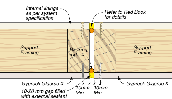
Figure 46: Vertical Control Joint – Tape
