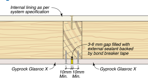
Figure 45: Vertical Junction – Sealant
