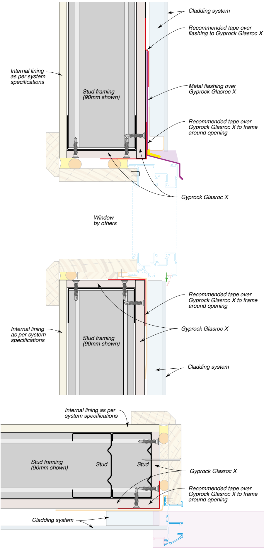
Figure 27: Window Penetration
