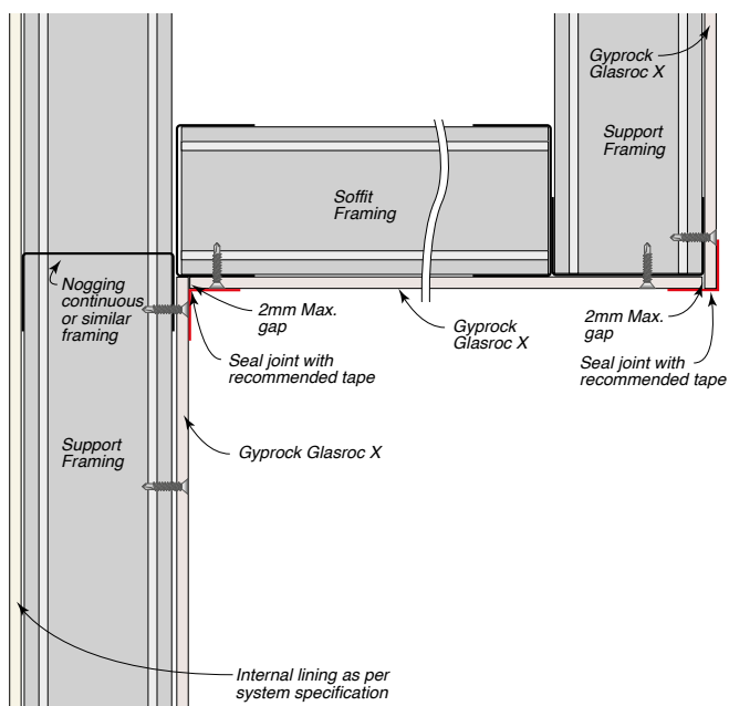
Figure 25: Soffit Junction – Tape
