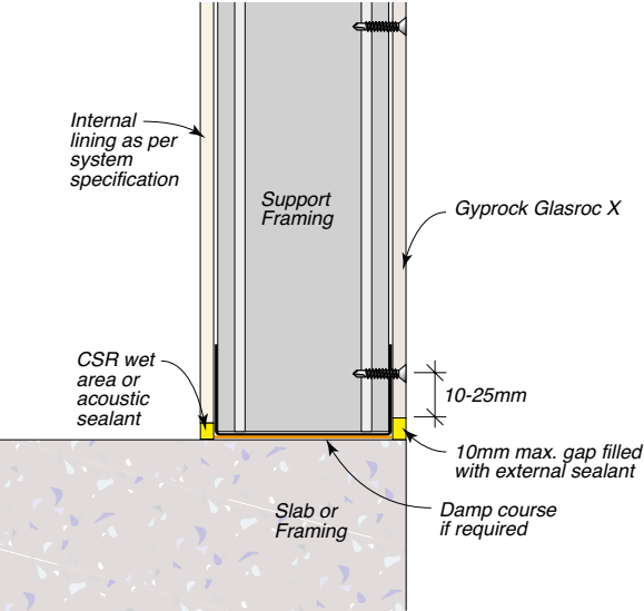
Figure 16: Base Detail – Sealant
