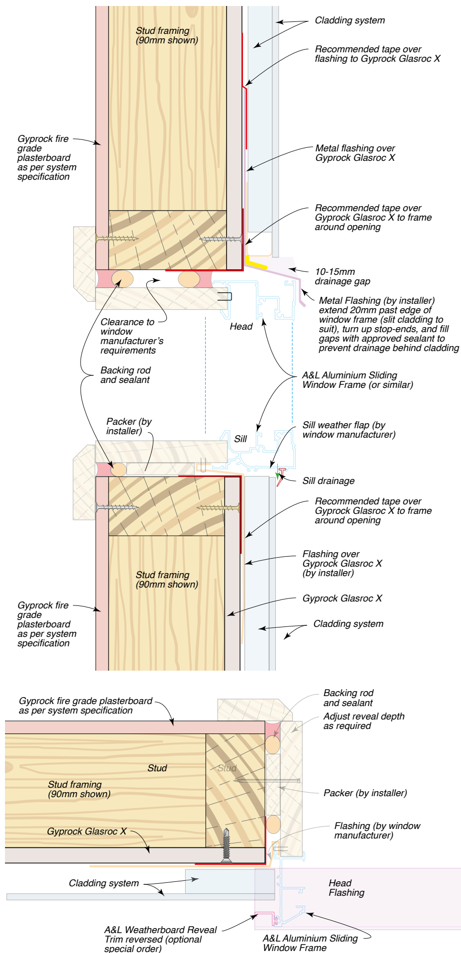
Figure 75: Window penetration
